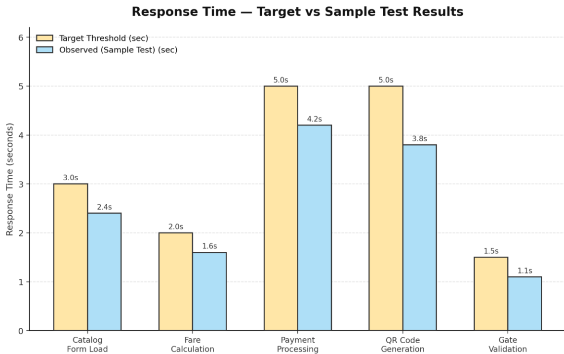
Figure 2 — Response Time: Target vs Sample Test Results
